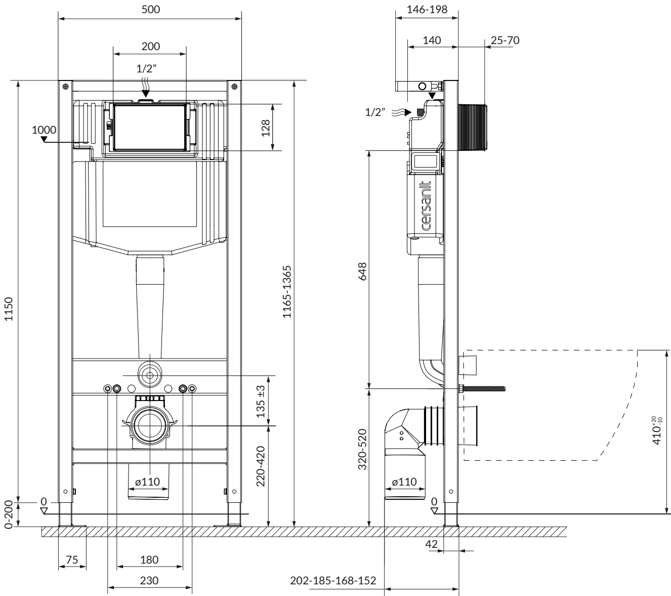
SYSTEM 50 MECHANICAL CONCEALED WC FRAME
