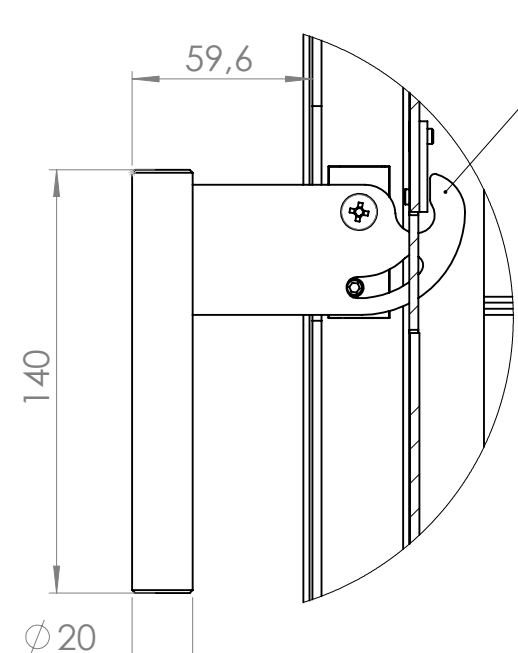
SECTION E-E SCALE 1 : 5
