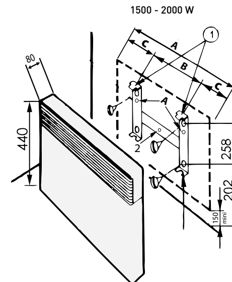
Fig. 1: Wandmontage
