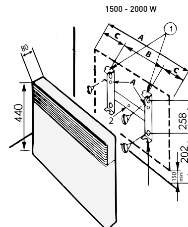
Fig. 1: Wall mounting:
