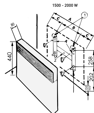
Fig. 1: Wandmontage
