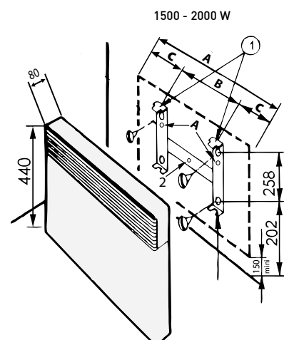
Fig. 1: Montage mural
