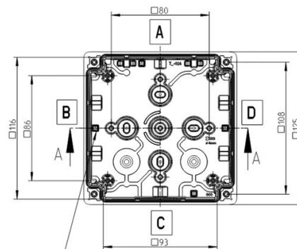
Innenansicht/interior view
