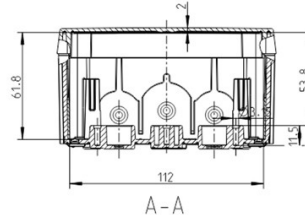
Innenansicht/interior view
