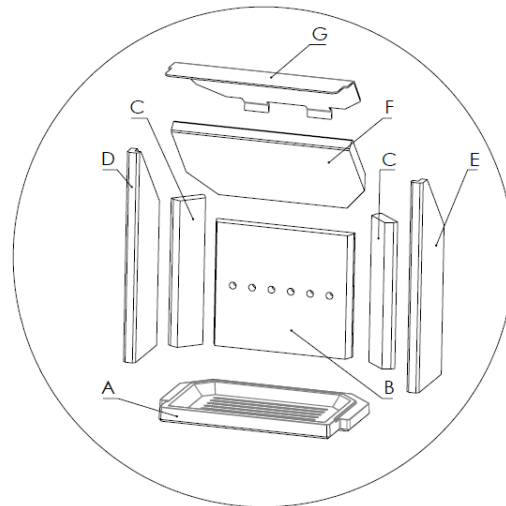
Figure 18 – Combustion chamber lining with grate
