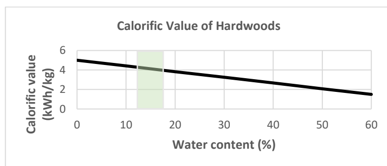
Figure 19 - Variation in calorific value depending on moisture content
