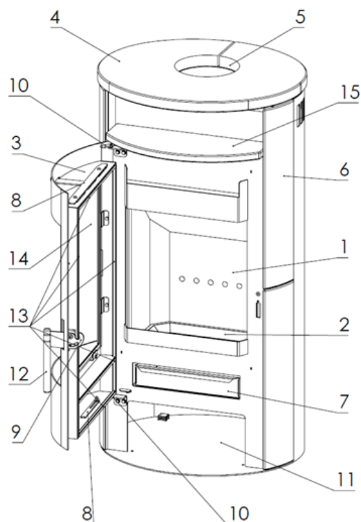
Figure 1 – Construction of the appliance
