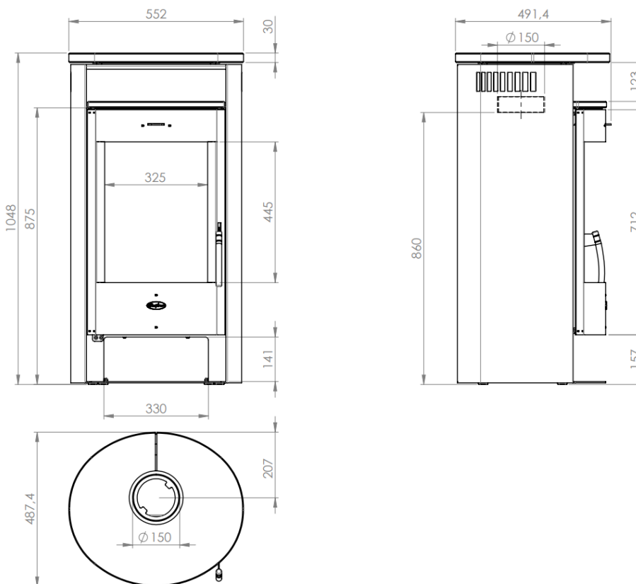
Figure 8 - Key Dimensions
