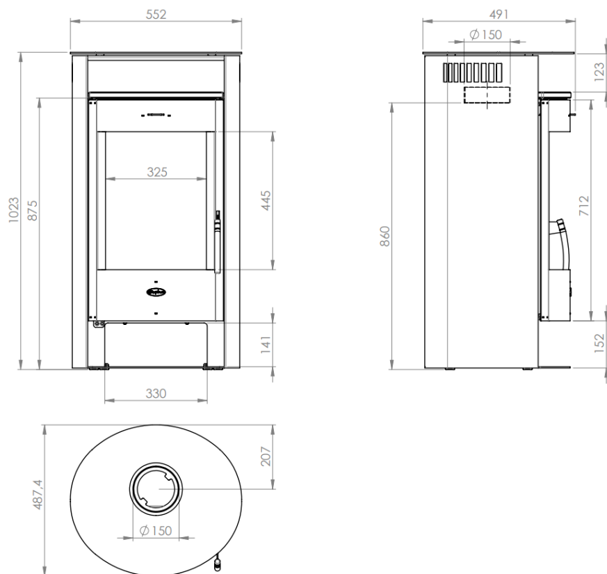
Figure 9 - Key Dimensions
