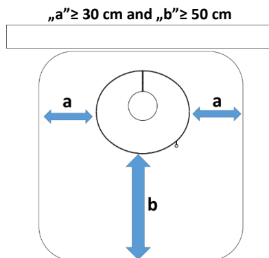
Figure 13 – Hearth plate
