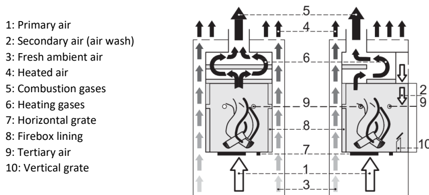
Figure 12 – Fire-Plus System, schematic diagram
