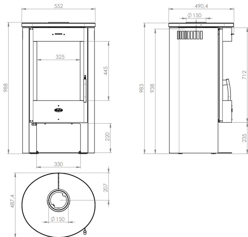
Figure 5 - Key Dimensions
