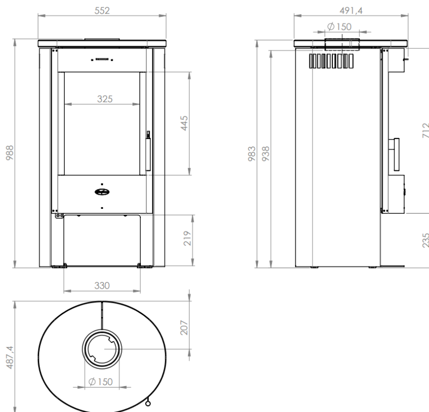
Figure 10 - Key Dimensions
