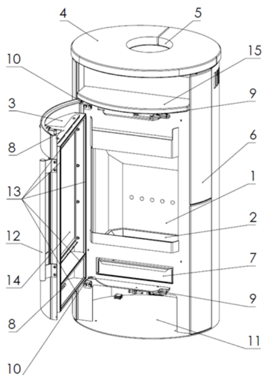
Figure 2 - Construction of the appliance /R5688 & R5693/
