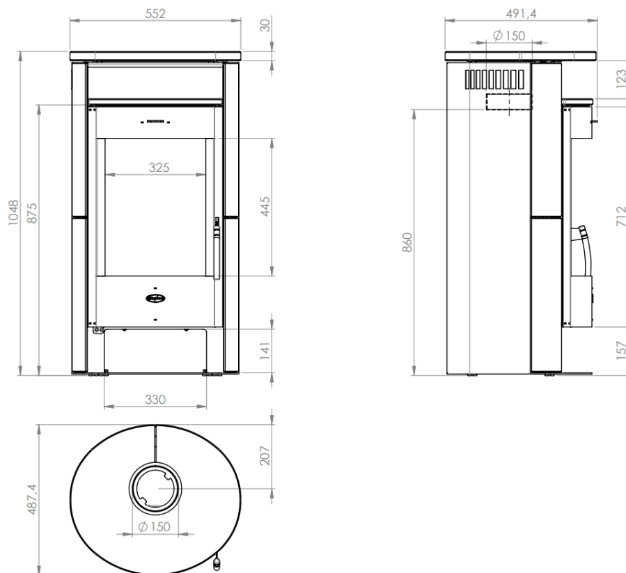
Figure 7 – Key Dimensions
