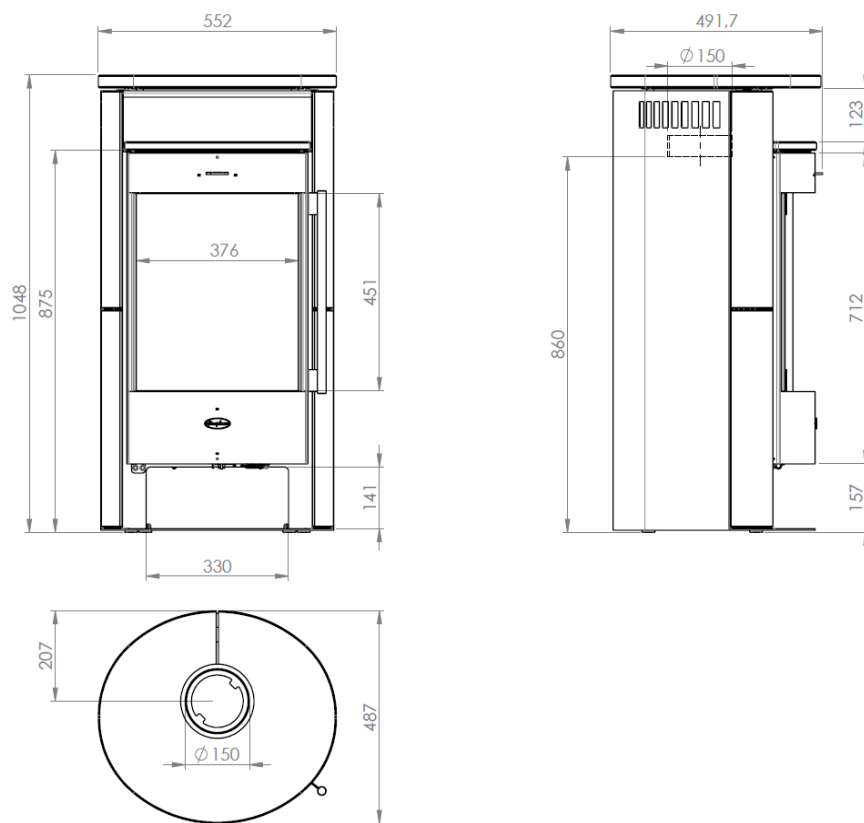
Figure 6 - Key Dimensions
