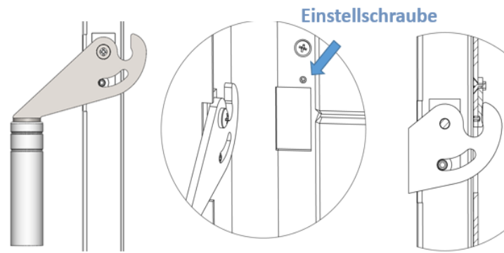
Figure 21 – Door lock
