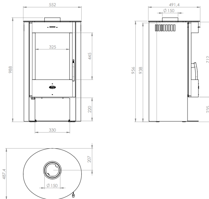
Figure 4 – Key Dimensions
