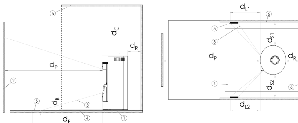
Figure 14 - Schematic representation of minimum distances (see Table 2)
