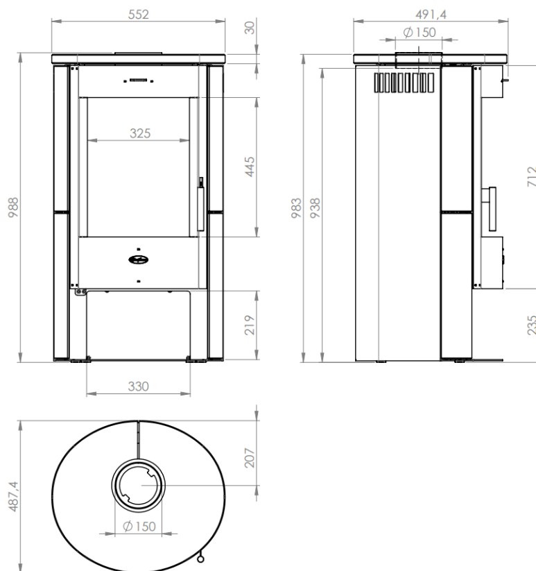
Figure 3 – Key Dimensions
