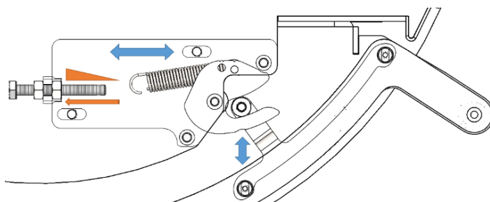
Figure 20 – Snap Lock (applies only to versions R5694 and R5696)
