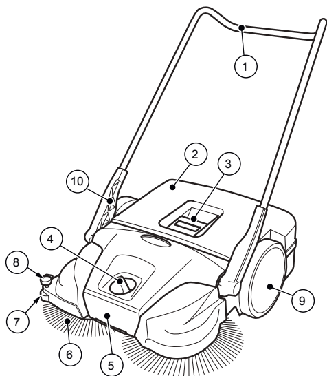
Fig. 1: Component overview 1
