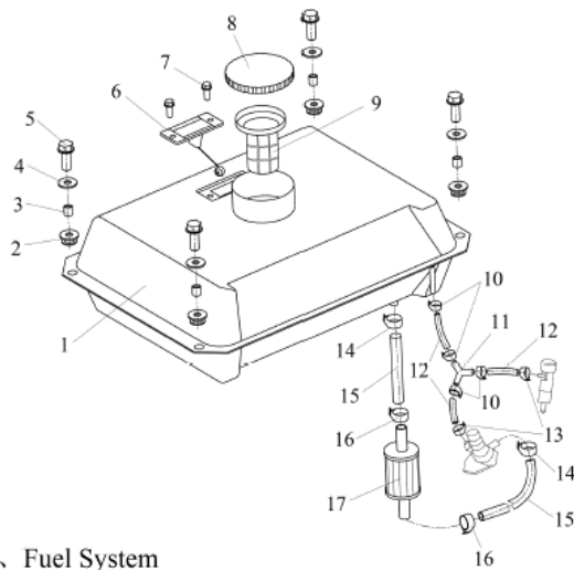
5、Fuel System
