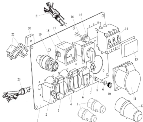
7、Panel Assembly
