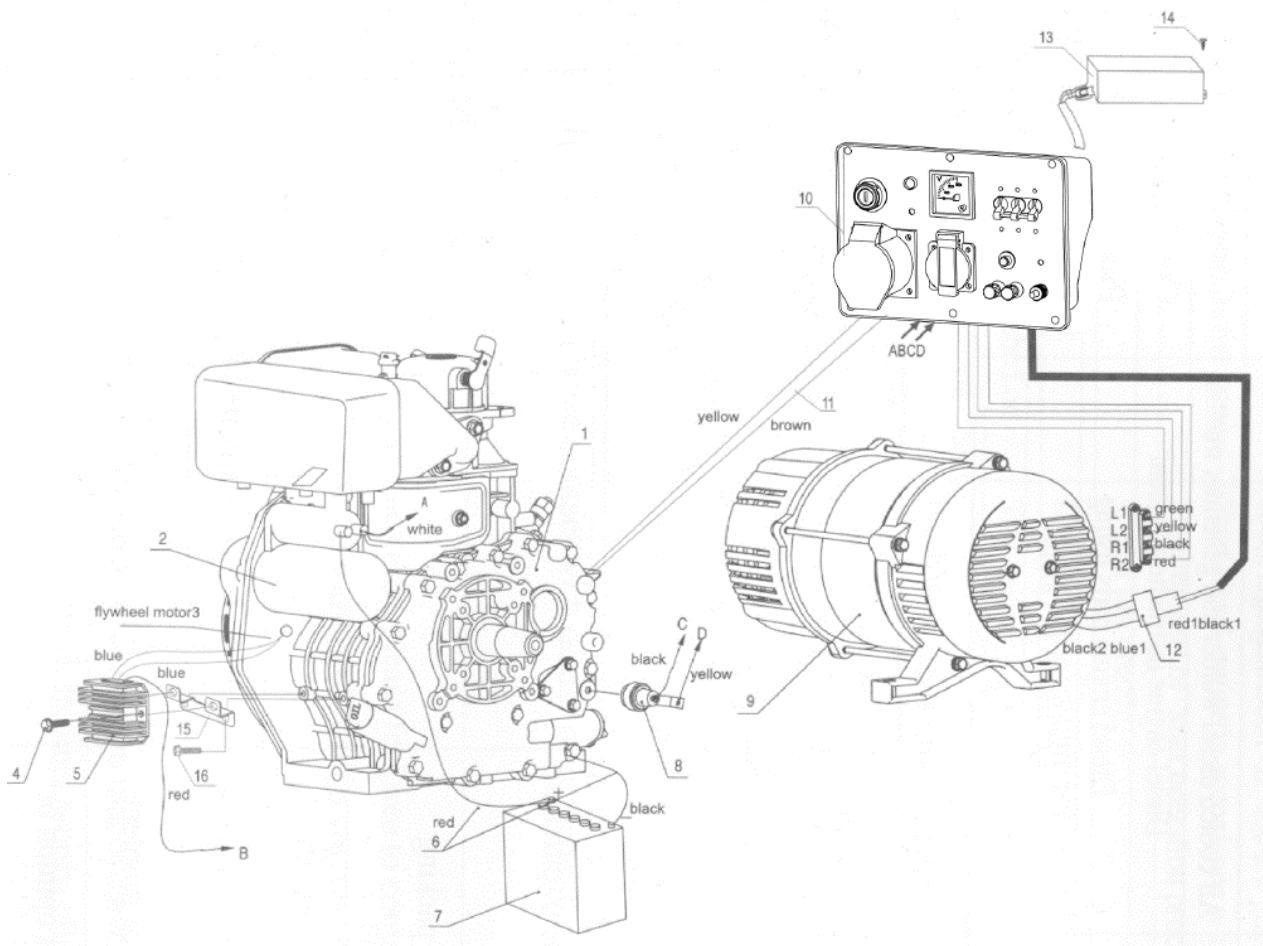
Engine-Generator Assembly
