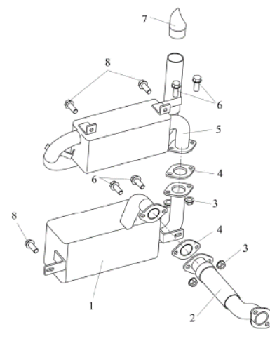
6、Muffler Assembly
