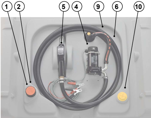
DT-Mobil Easy 440I with pump 12 V 40 l/min
