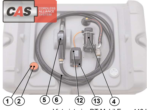
Vista interior DT-Mobil Easy 440 I
